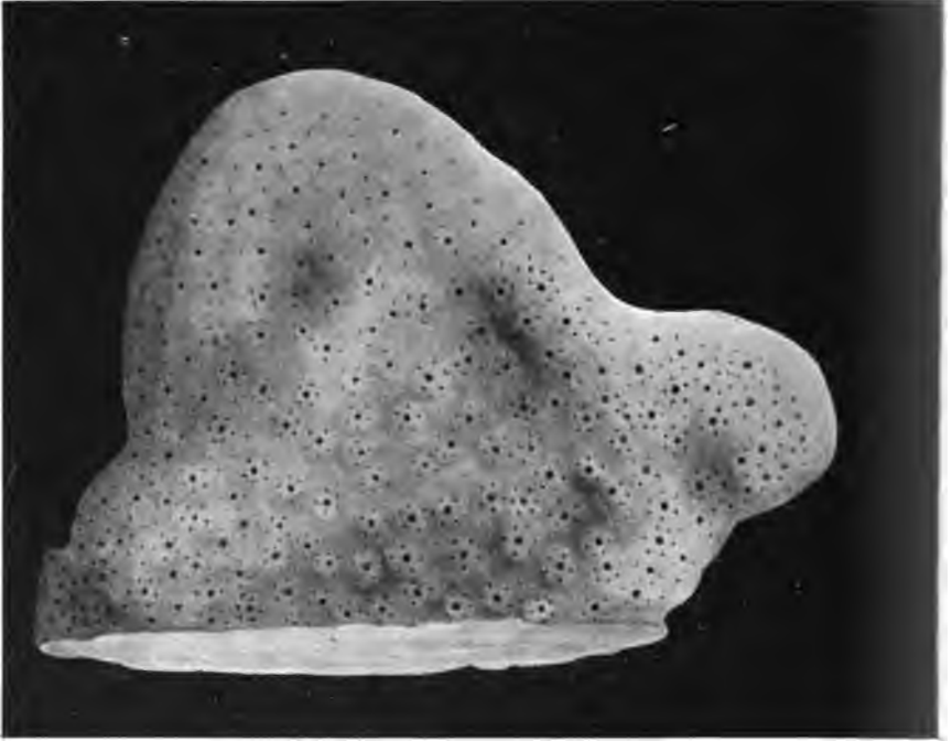
FIG. 128.—A portion of a dried colony of Millepora , showing the larger pores (gastropores) surrounded by cycles of smaller pores (dactylopores). At the edges the cycles are not well defined.
